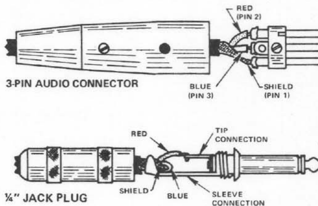
FIGURE 5 – 3-Pin Connector & 1/4" Jack Plug Wiring Connections
