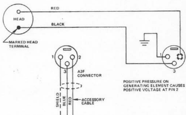
FIGURE 2 – Wiring Diagram
