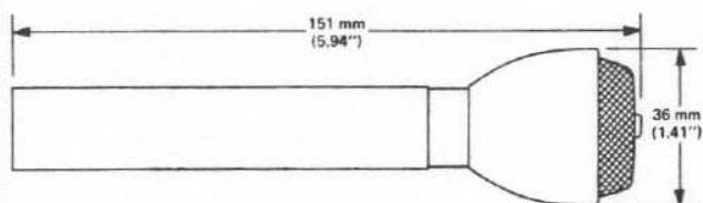
FIGURE 1 – Dimensions
